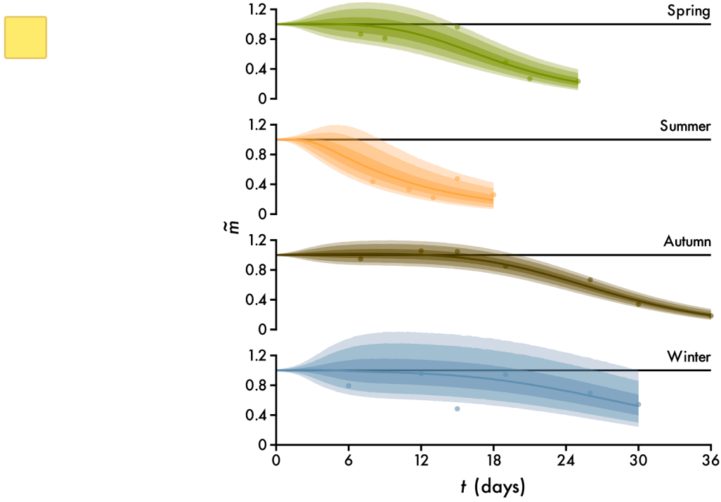
Fig. 4. Example 3: the effect of season on the decomposition of Ulvaria obscura , shown as normalised remaining mass over time t ( n = 28 , data from Bourguès et al. 1996). Data are plotted alongside predictions of new observations \bar{m} (Eq. 18, cf. Fig. S4). Lines and intervals are medians and the central 50, 80 and 90% of posterior probability.
