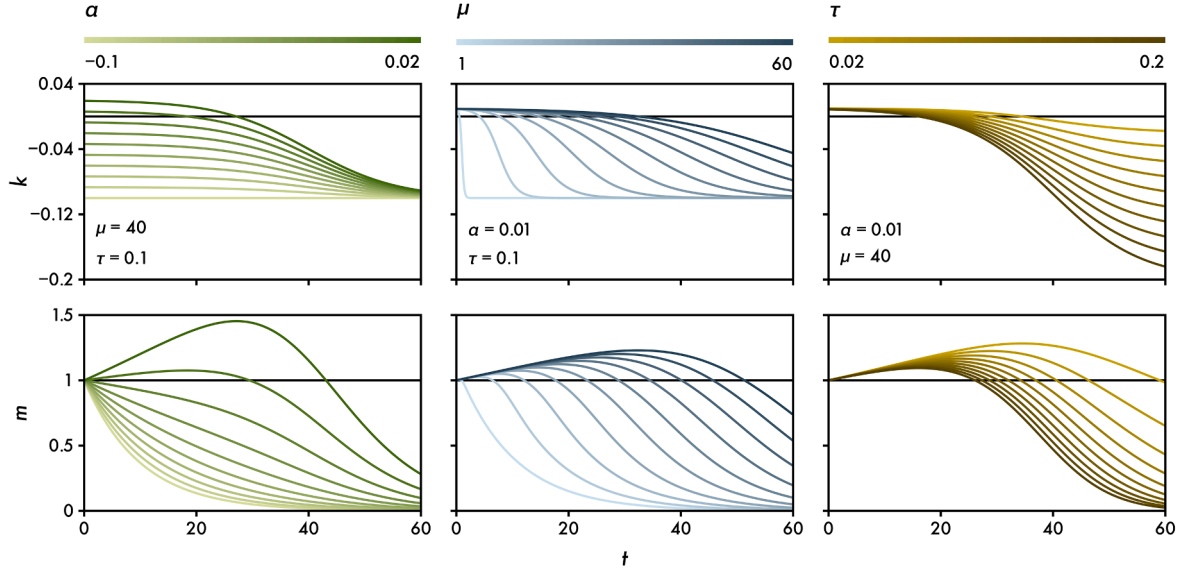
Fig. 1. The mathematical model: the effect of varying \alpha , \mu and \tau on the trajectory of the exponential rate k (Eq. 6) and normalised remaining mass m (Eq. 9) over time t (cf. Fig. S1).
