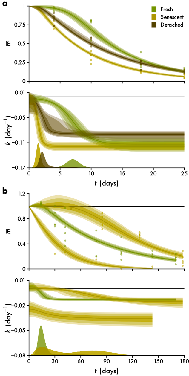
Fig. 3. Example 2: the effect of senescence on the decomposition of Macrocystis pyrifera (a, n = 61 , data from Hamersley et al. 2015) and Laminaria hyperborea (b, n = 63 , data from de Bettignies et al. 2020), shown as normalised remaining mass over time t . Data are plotted alongside predictions of the mean \bar{m}_i , the time-variant exponential rate k and photosynthetic half-life \mu (Eqs. 16 and 17, cf. Fig. S3). Lines and intervals are medians and the central 50, 80 and 90% of posterior probability. Distributions are kernel density estimates of the probability density function of \mu .
